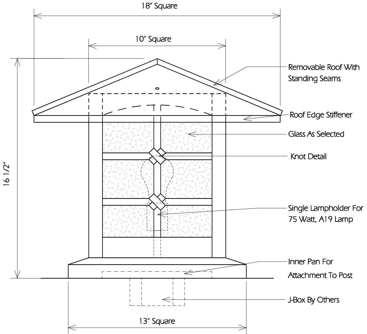
TYPICAL SIDE
