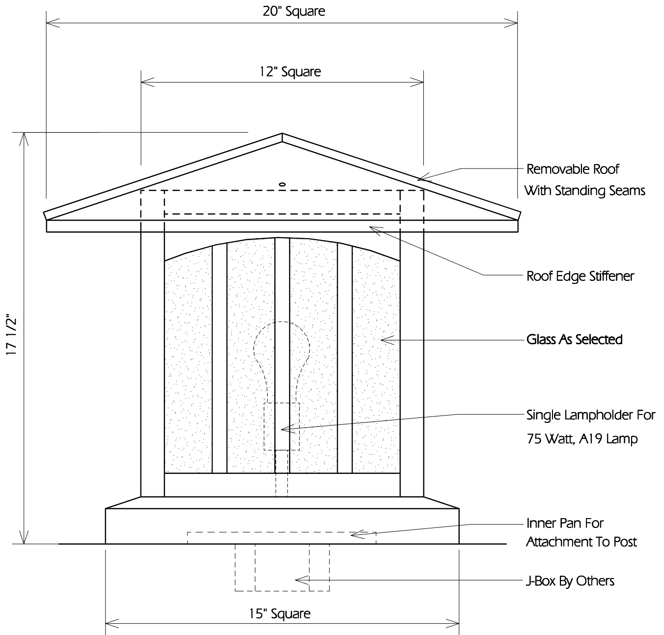
TYPICAL SIDE
