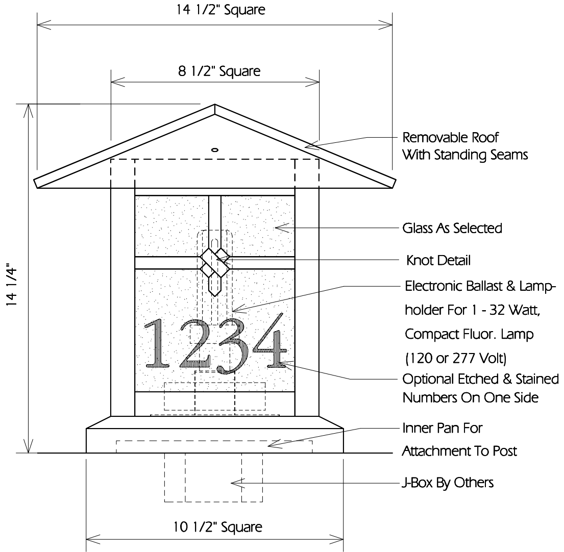
TYPICAL SIDE
