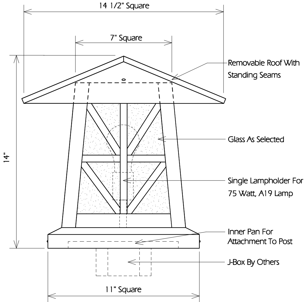
TYPICAL SIDE
