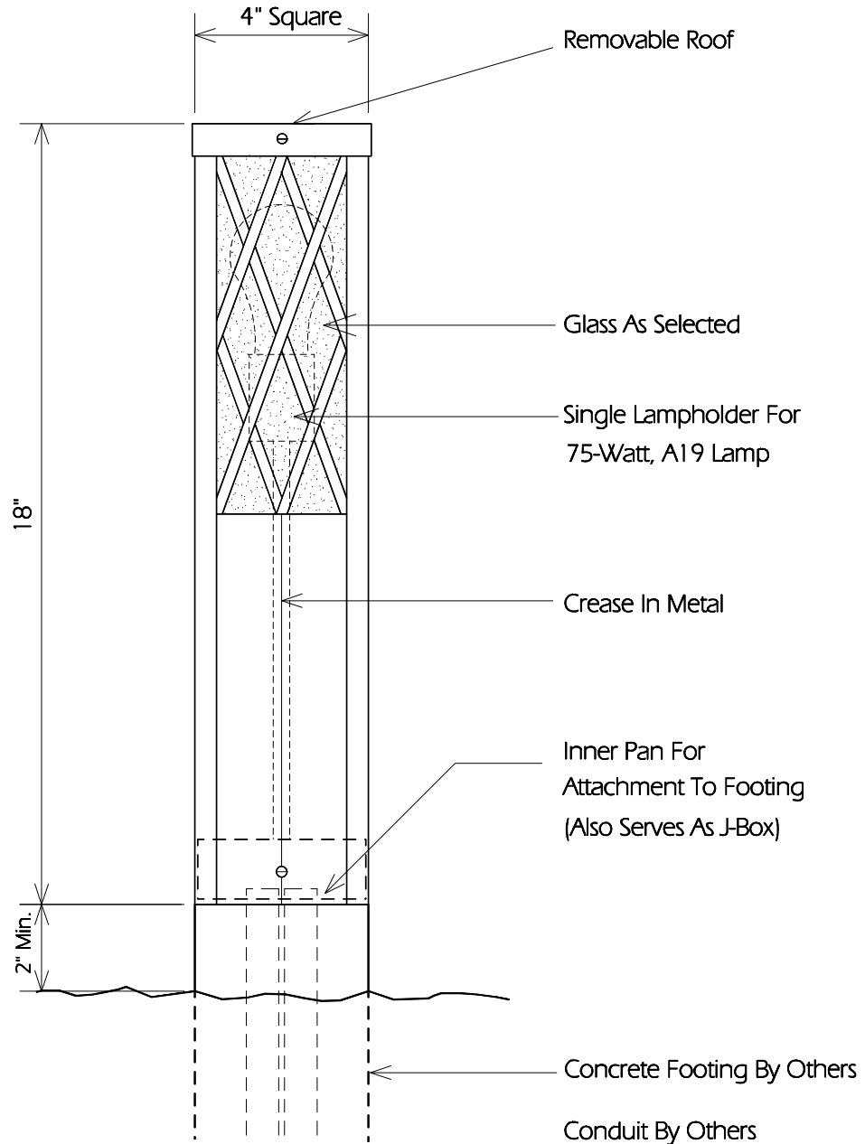
TYPICAL SIDE
