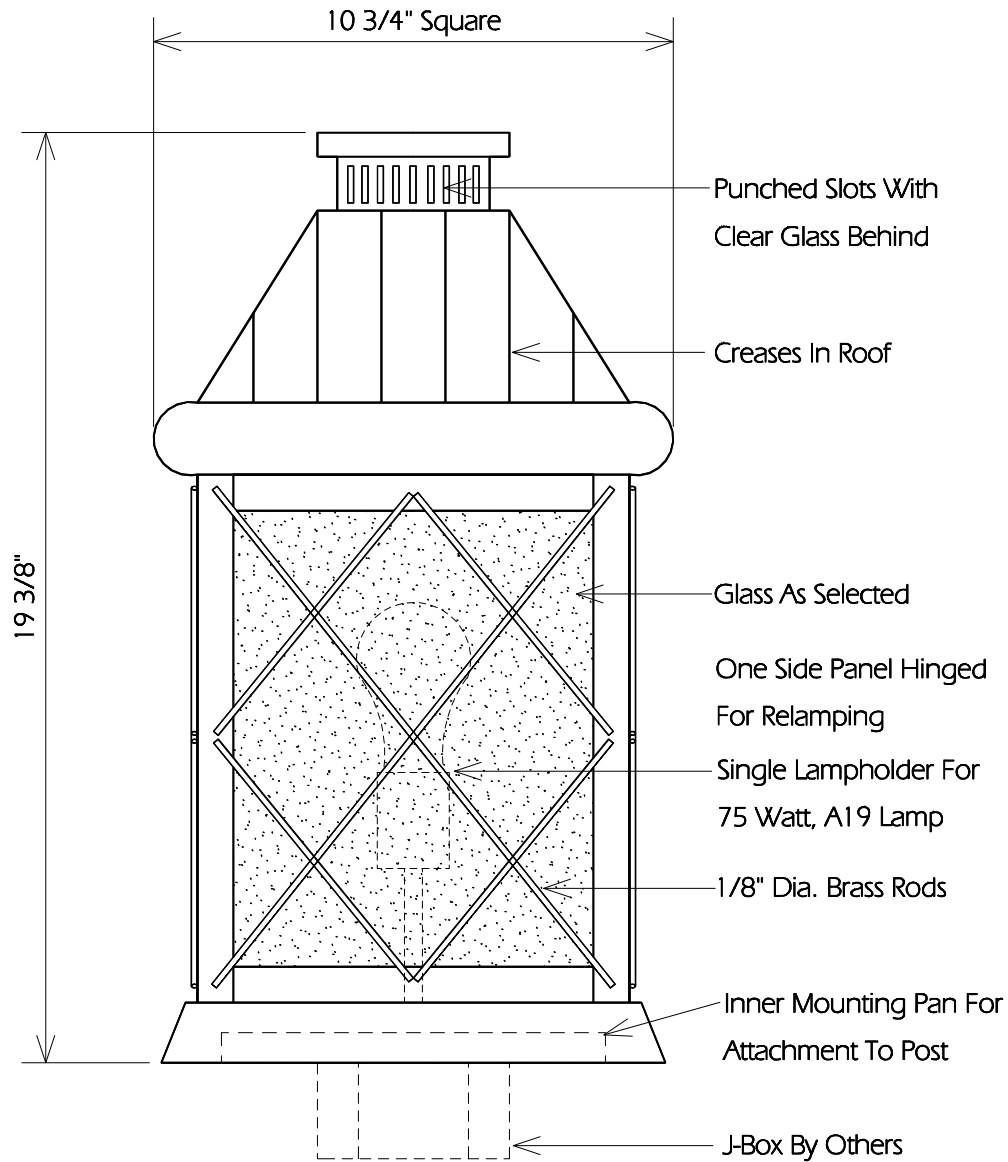
TYPICAL SIDE
