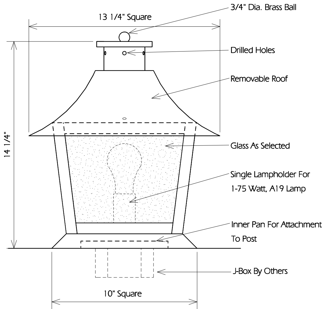
TYPICAL SIDE
