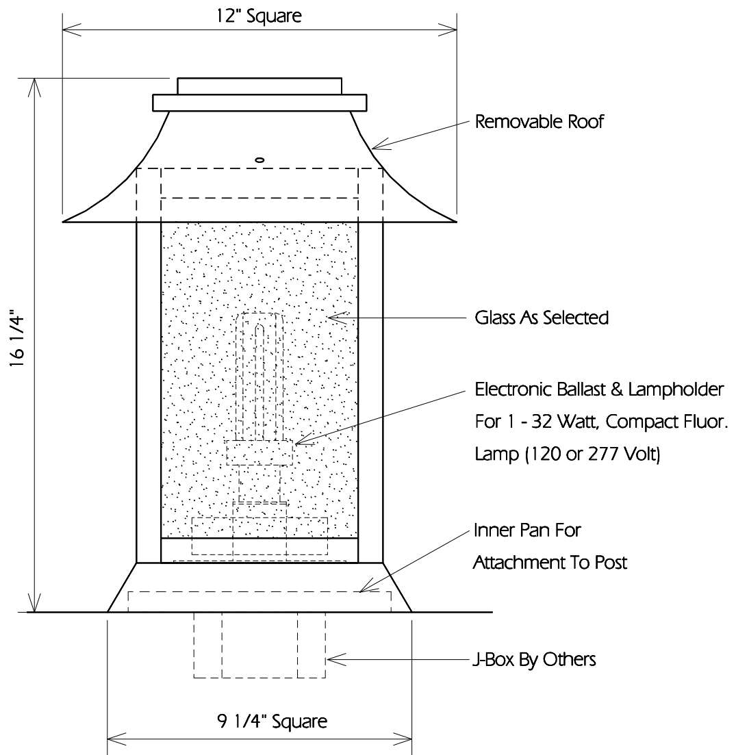
TYPICAL SIDE
