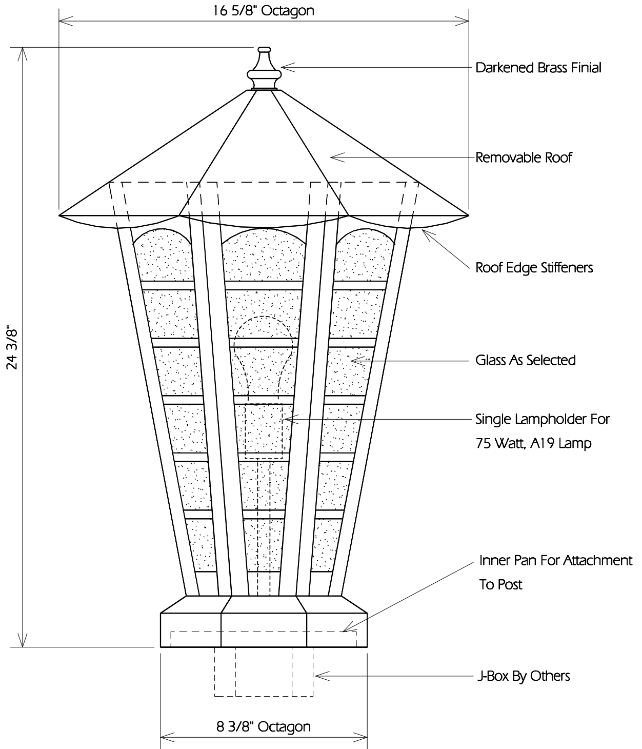
TYPICAL SIDE
