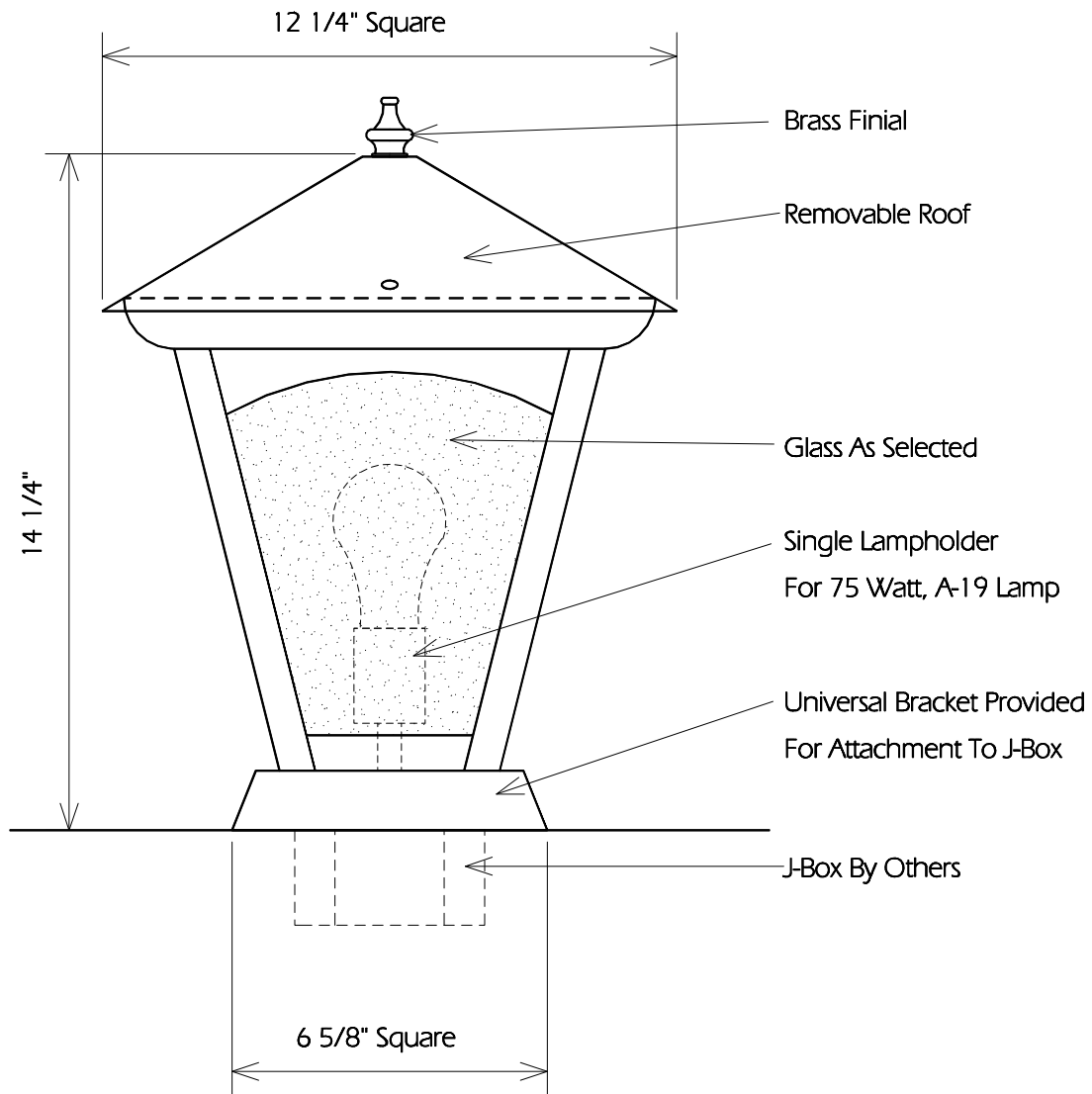
TYPICAL SIDE
