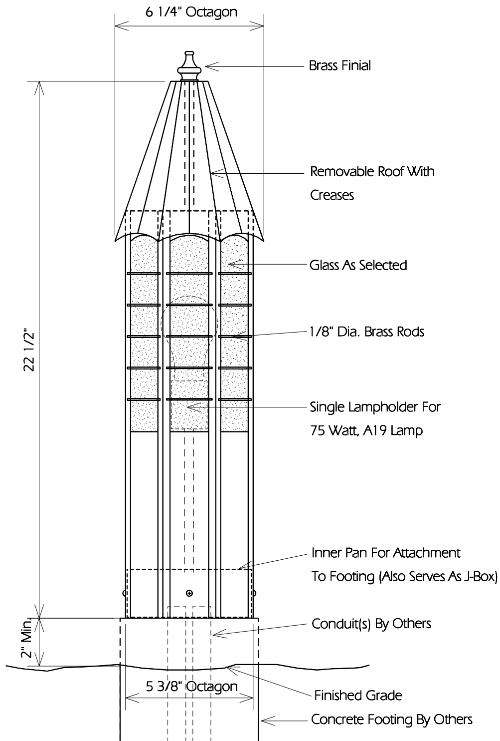
TYPICAL SIDE
