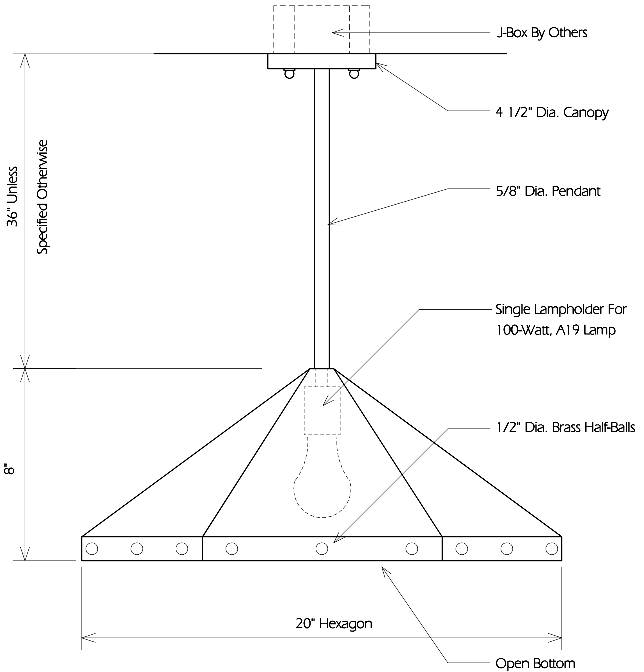
TYPICAL SIDE
