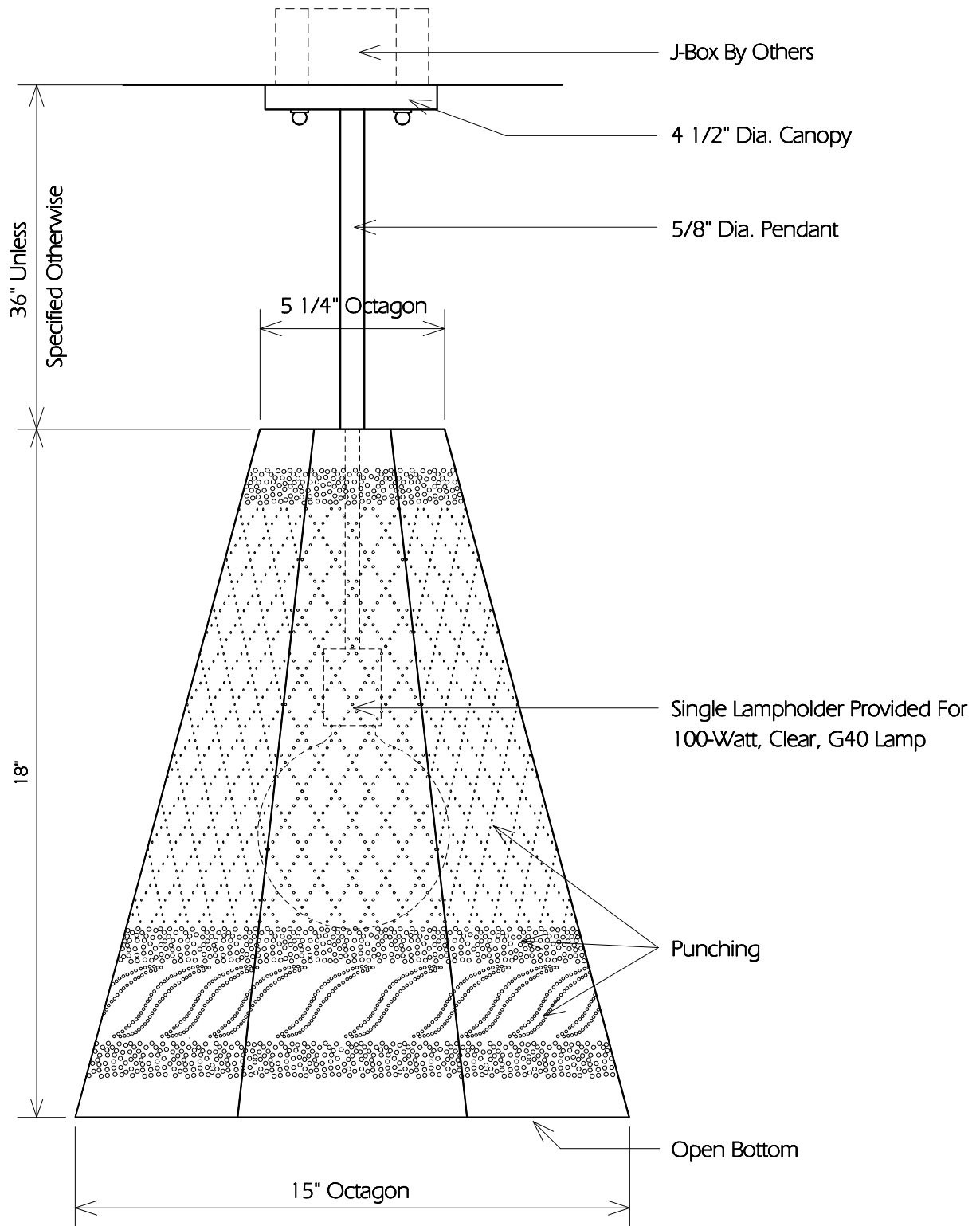
TYPICAL SIDE
