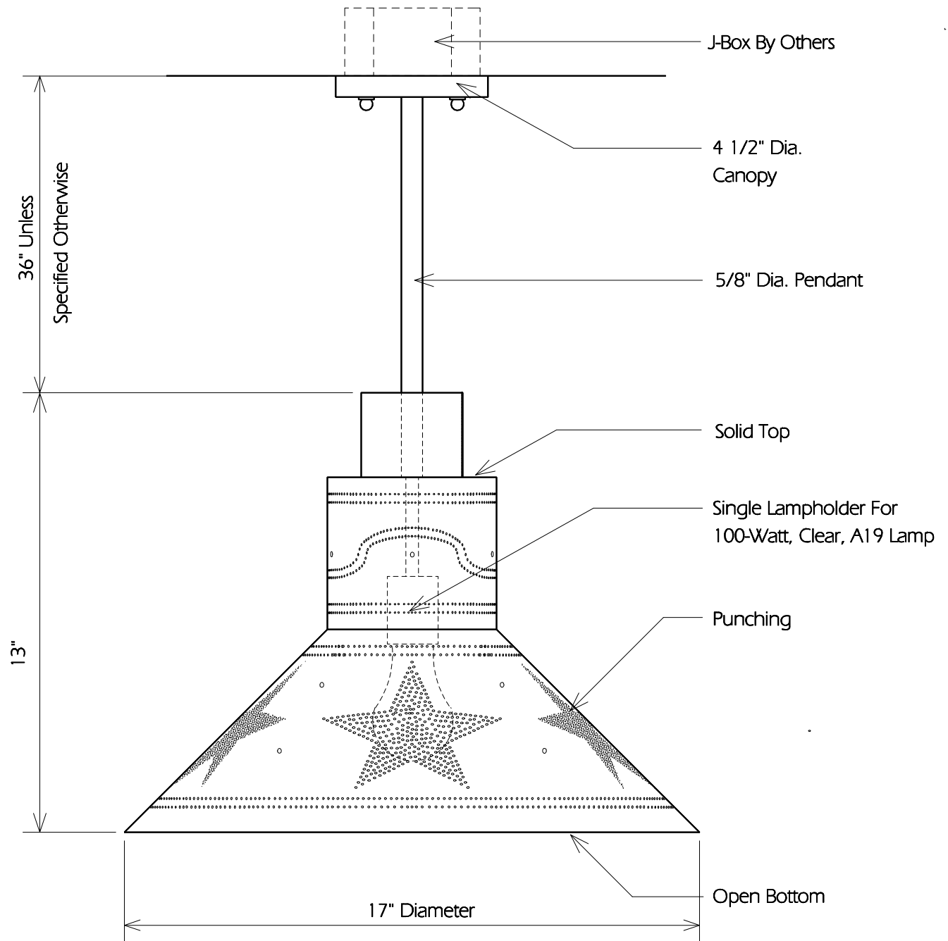
TYPICAL SIDE
