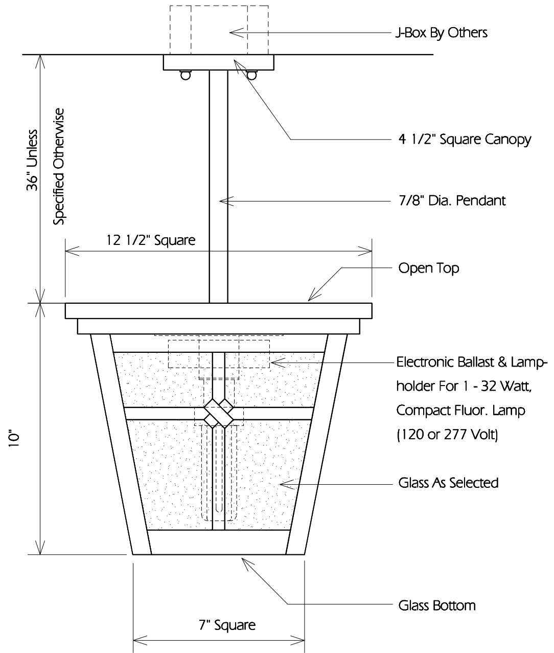
TYPICAL SIDE
