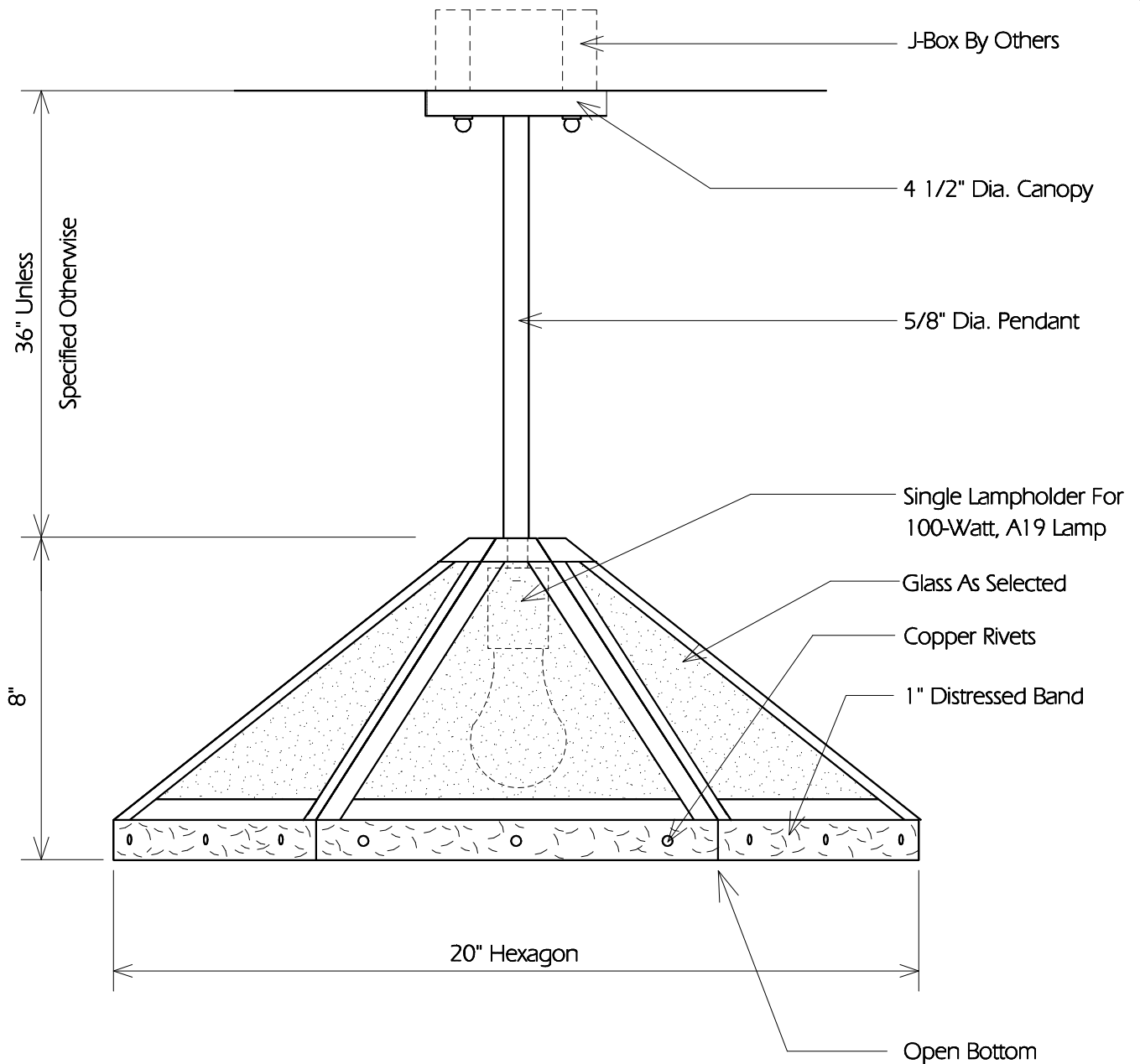
TYPICAL SIDE
