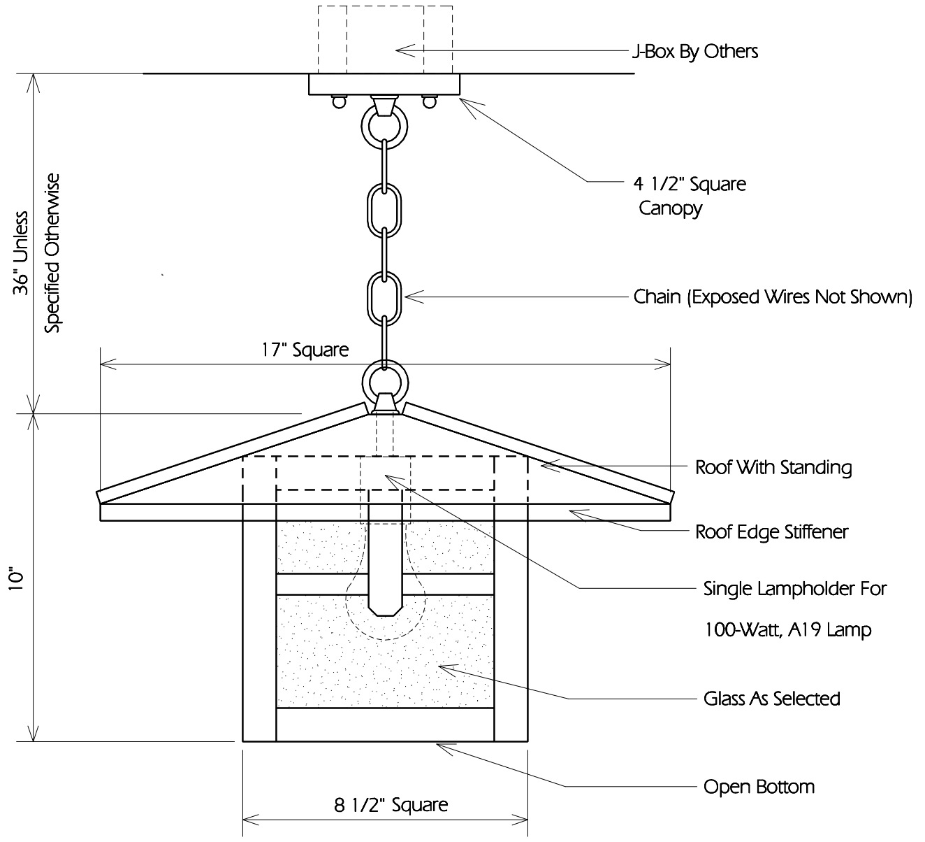
TYPICAL SIDE
