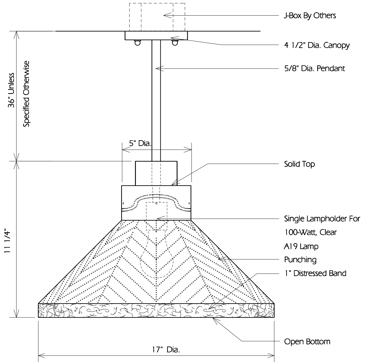
TYPICAL SIDE
