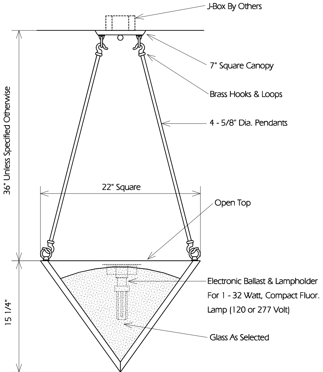
TYPICAL SIDE
