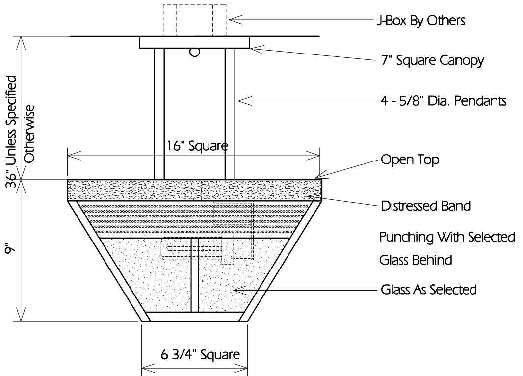
SIDE
