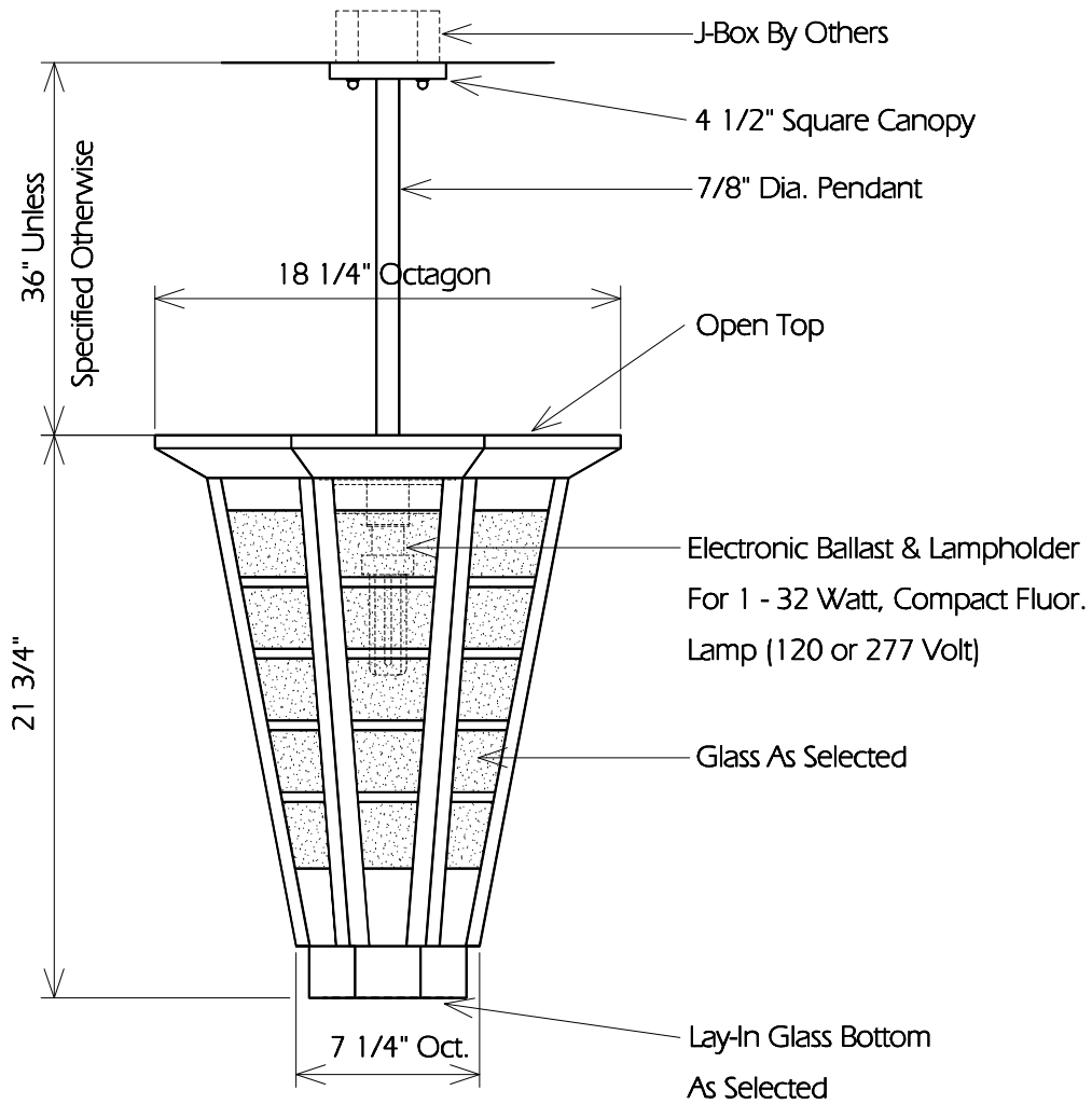
SIDE
