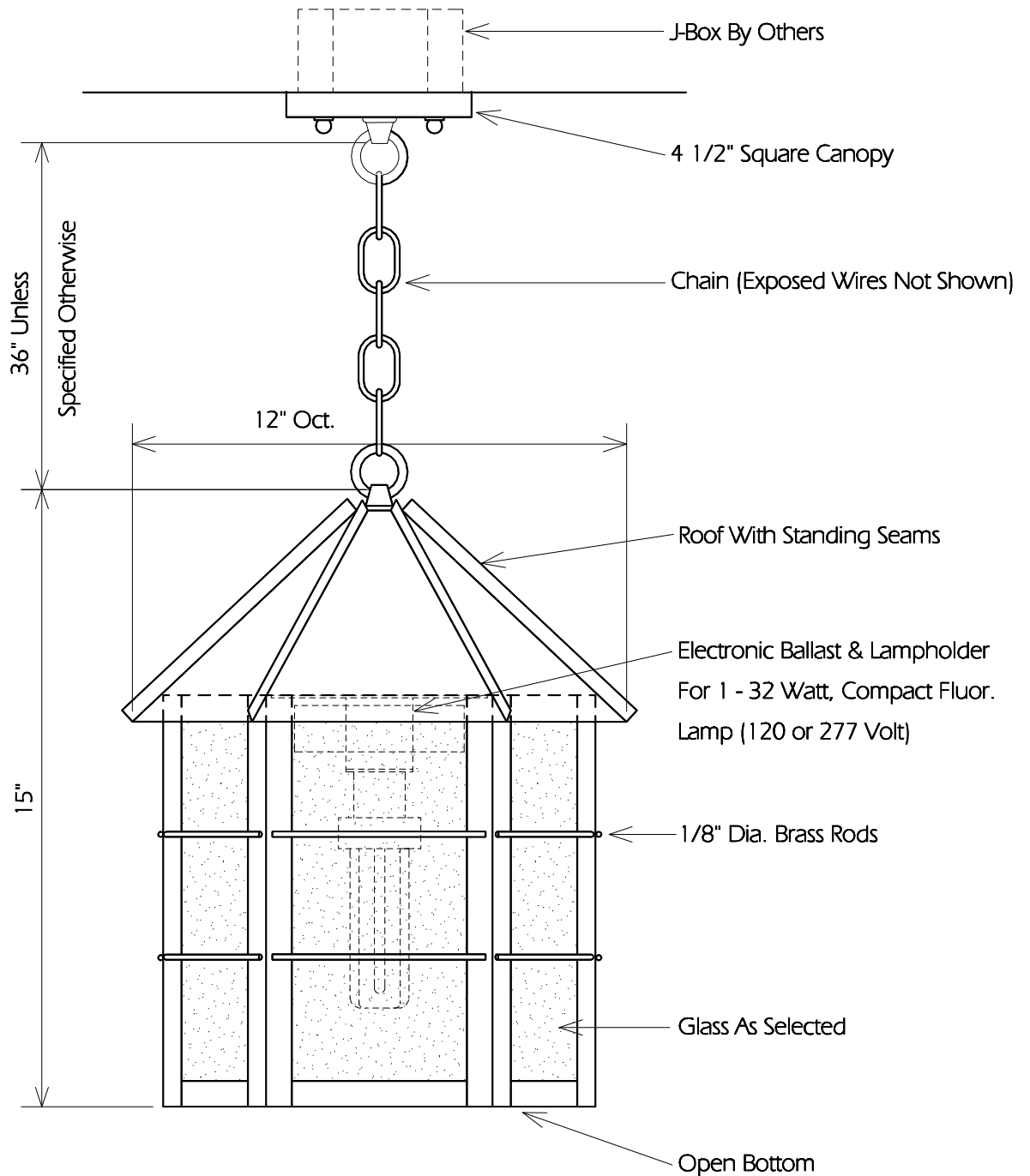
TYPICAL SIDE
