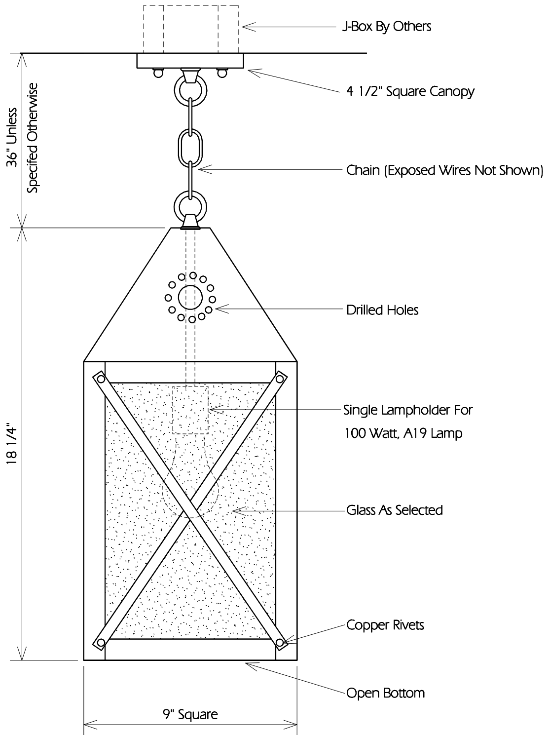
TYPICAL SIDE
