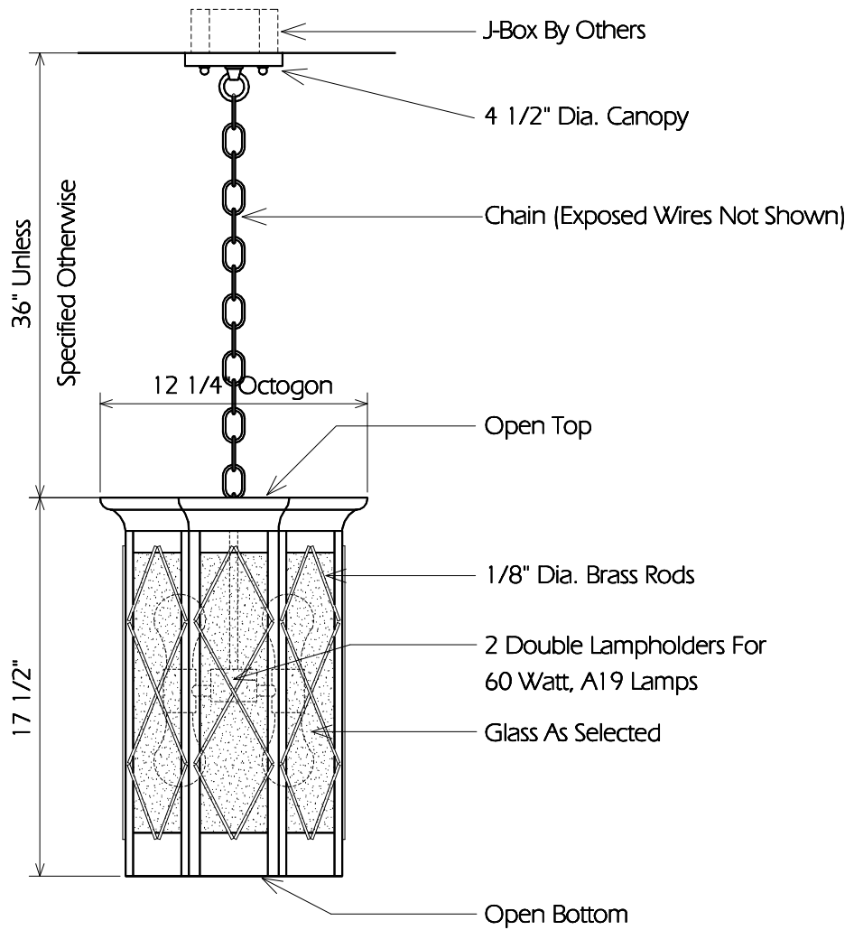
TYPICAL SIDE
