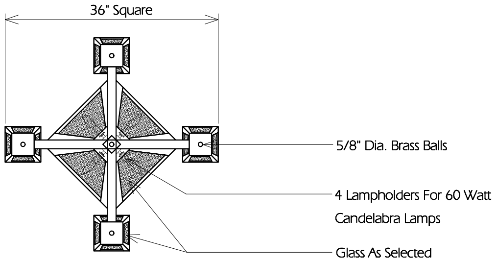
BOTTOM (Shown At Half Size)
