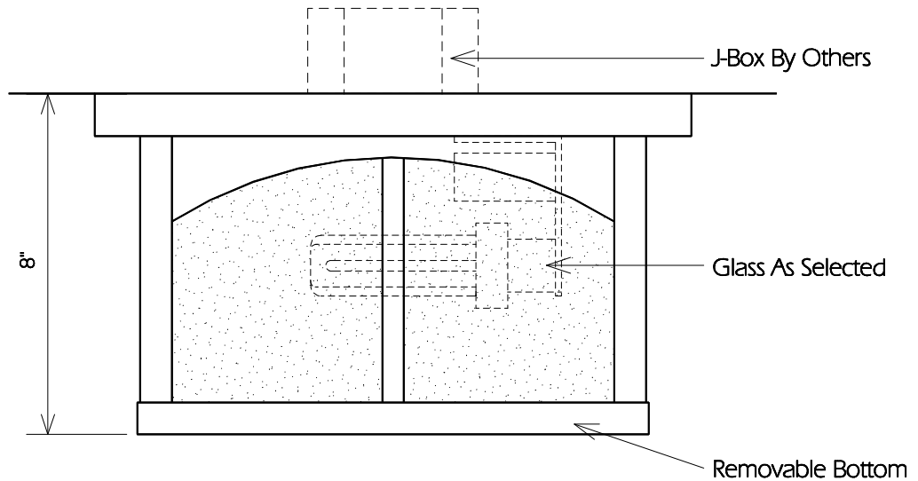
TYPICAL SIDE
